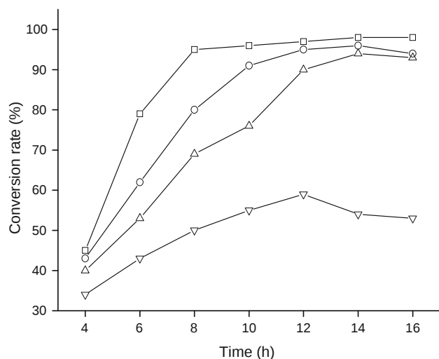
Fig. 3 Conversion rate time course of DL-threo - \beta -(methylsulfonylphenyl) serine. The reaction was carried out in a 10 ml mixture containing 1 g immobilized SHMT cells at pH 7.5. The DL-threo - \beta -(methylsulfonylphenyl) serine concentrations were 50 mmol/l (□), 100 mmol/l (○), 200 mmol/l (Δ), and 400 mmol/l (▽) respectively. The mixture was kept at 45°C as it was being shaken
